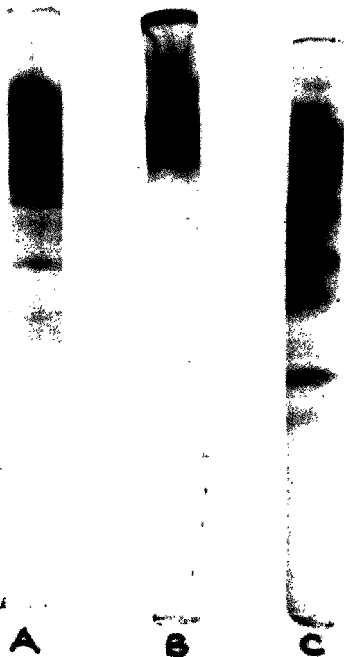
Fig.2. Polyacrylamide gel electrophoresis of MetRS fractions: 70 (gel A), 95 (gel C) and 100 (gel B) from the fig.1.
